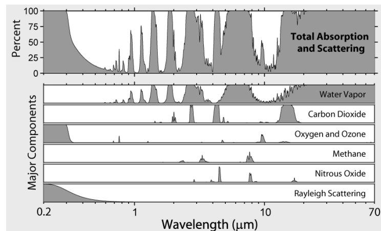
FIGURE 2. Transmission “windows” versus laser wavelength. [4]
