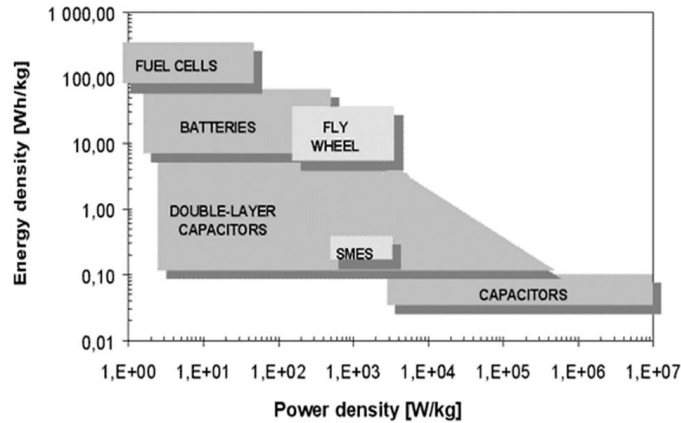
FIGURE 5. Energy density versus power density for various energy storage alternatives [4].
